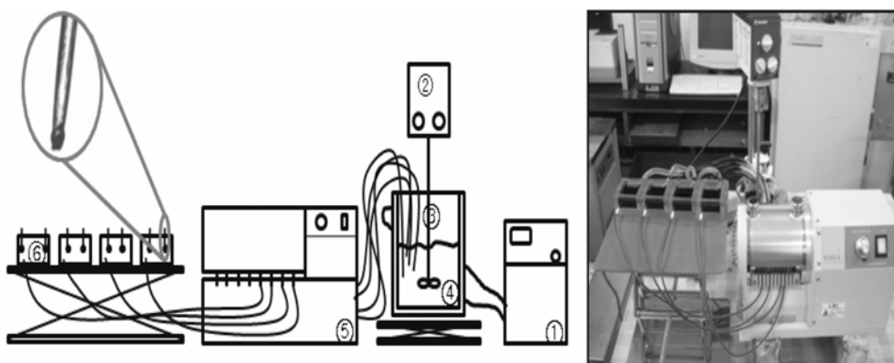
Fig. 2. Schematic apparatus (① Heating bath, ② Agitator, ③ Propeller, ④ Double jacket, ⑤ Micro Tubing Pump, ⑥ 16 ml reactor).
